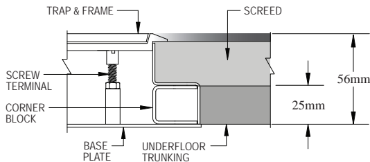
FLOOR BOX DEPTH
