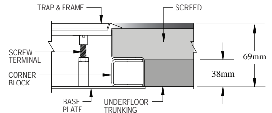
FLOOR BOX DEPTH
