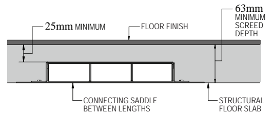
SCREEDING DEPTH
