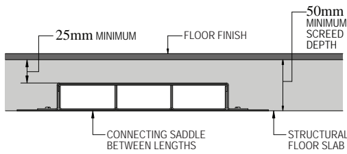
SCREEDING DEPTH
